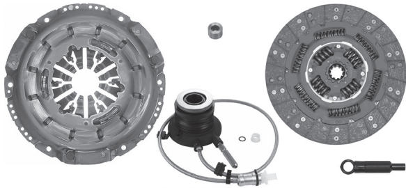
EJ-GM30H 298mm (11 3/4") - 23.2 x 28.8mm / 10D Autoajustable
