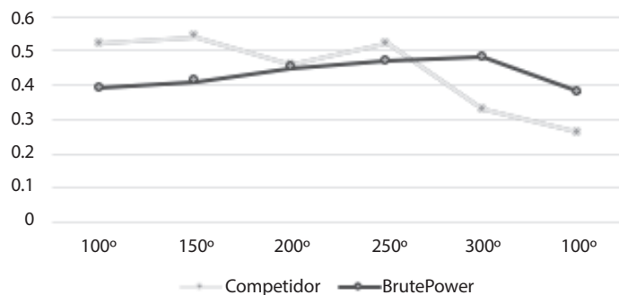
Friction Coefficient Test
